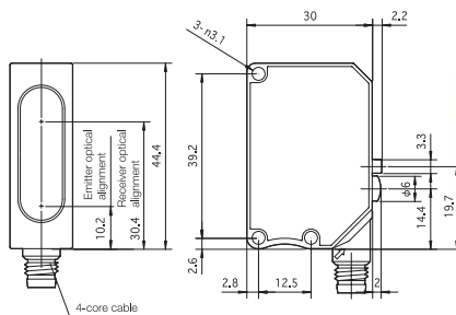
Connector type sensor
